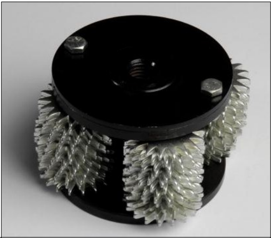
2" Star Cutter Hub Assembly Part No. 438.0220
